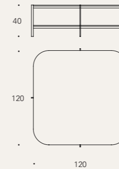
Top: 120x120 cm Metal leg (1): 2,5 cm Final size: 125x125 cm
