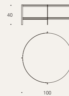
Top: Ø100 cm Metal leg (1): 2,5 cm Final size: Ø105 cm
