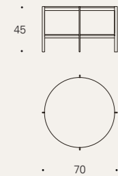
Top: Ø70 cm Metal leg (1): 2,5 cm Final size: Ø75 cm
