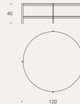
Top: Ø120 cm Metal leg (1): 2,5 cm Final size: Ø125 cm
