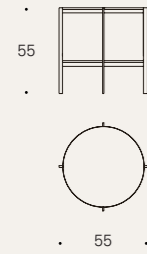
Top: Ø55 cm Metal leg (1): 2,5 cm Final size: Ø60 cm
