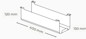
AKIF012210C
